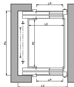
2 accessi opposti
