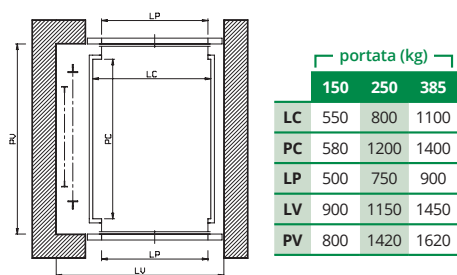
2 accessi opposti
